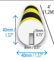
Half Circle I-Beam Protector Part #: HCIB120 Quantity / Pack: 1
