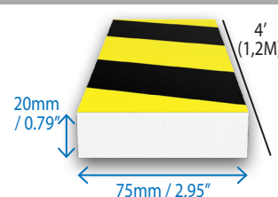
Large Rectangle Surface Bumper Part #: LRSB120 Quantity / Pack: 1
