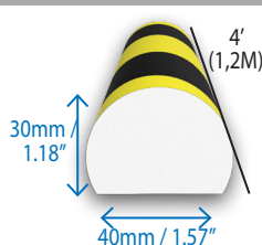
Round Surface Bumper Part #: RDSB120 Quantity / Pack: 1
