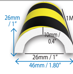
Half-Circle Pipe Bumper Part #: HCPB100 Quantity / Pack: 1
