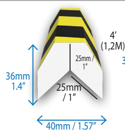
Conic Corner Bumper Part #: CCP120 Quantity / Pack: 1
