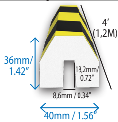
Conic I-Beam Protector Part #: CIBP120 Quantity / Pack: 1
