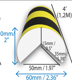
Large Round Corner Bumper Part #: LRCB120 Quantity / Pack: 1
