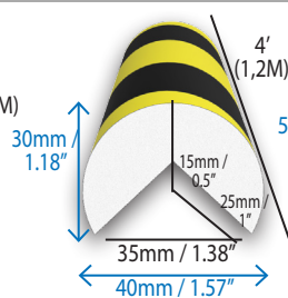
Round Corner Bumper Part #: RCB120 Quantity / Pack: 1
