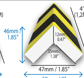
Large Square Corner Bumper Part #: LSCB120 Quantity / Pack: 1
