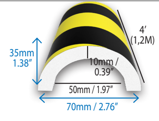
Large Half-Circle Pipe Bumper Part #: LHCPB120 Quantity / Pack: 1
