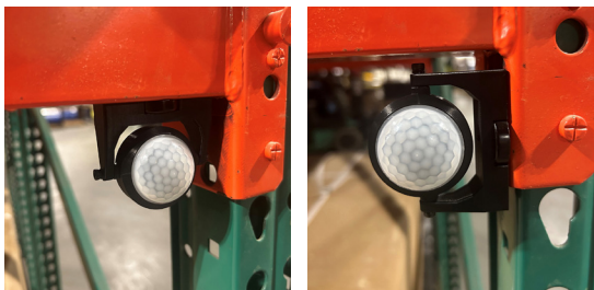
Motion Sensor can be installed on vertical or horizontal surface.
